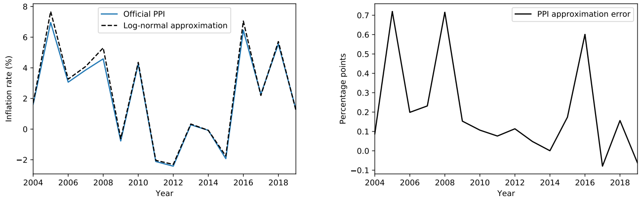
Figure 33: Annual inflation rates as measured by the baseline goods PPI and the log-normal approximation with \sigma_g = 0 and \sigma = 0 (left figure), and their difference (right figure).
